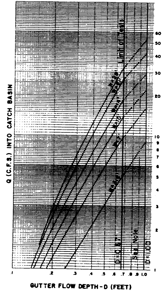
4" GUTTER DEPRESSION
