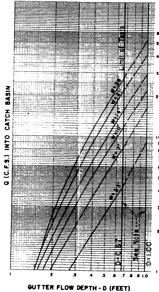
2" GUTTER DEPRESSION
