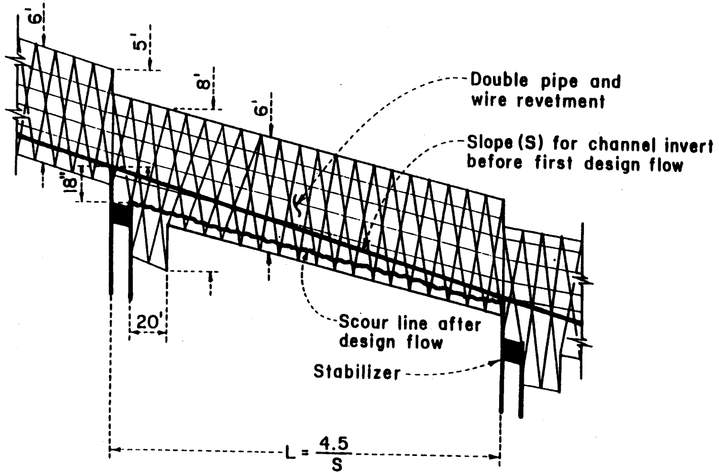
STABILIZER SPACING FOR CHANNEL WITH REVETMENT NOT TO SCALE
