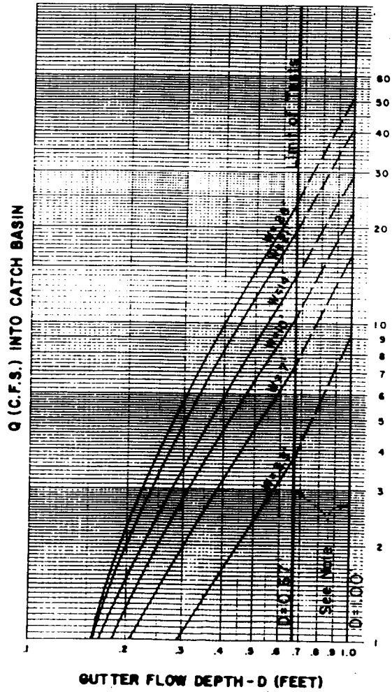
1" GUTTER DEPRESSION
