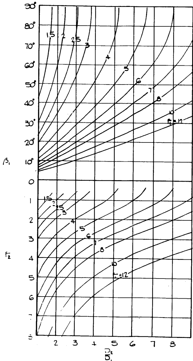
General relations between F_1, \theta, \beta, D_2/D_1 and F_2
