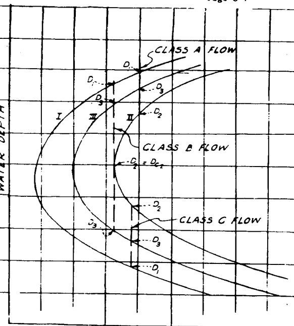
PRESSURE+MOMENTUM CURVES
