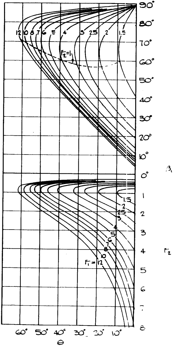
General relations between F_1, \theta, \beta, D_2/D_1 and F_2
